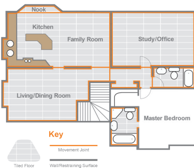
An example of movement joint good practice
