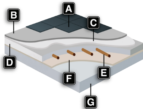
A - Tiles B - S1/ S2 Tile Adhesive C - Primer D - Calcium Sulfate Screed E - Heating Pipes F - Insulation G - Concrete Substrate
