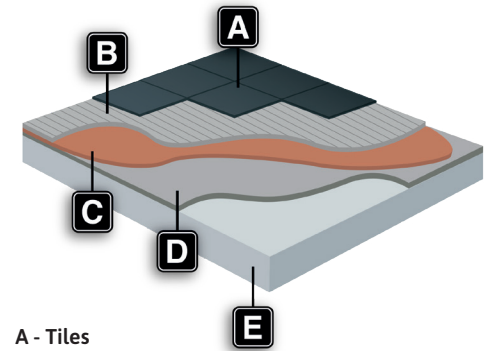
A - Tiles B - Tile Adhesive C - Uncoupling D - Levelling Screed E - Concrete Substrate
